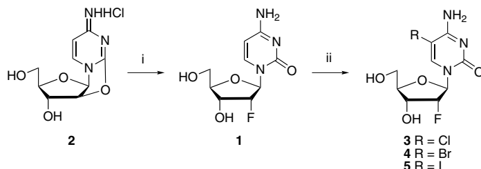
Scheme 1. Reagents and conditions: (i) KF, dibenzo[18]crown-6, DMF, 120 °C, 4 h; (ii) BzCl, m -CPBA, DMF, rt, 30 min; or pyridine, Br 2 , CCl 4 , rt, 25 min; or MeOH, ICl, 50 °C, 4 h.
