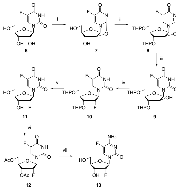
Scheme 2. Reagents and conditions: (i) HMPA, Ph 2 CO, NaHCO 3 , 135 °C, 40 min; (ii) DMF, 3,4-dihydro-2H-pyran, p -TsOH, 0 °C, 4 h; (iii) NaOH, MeOH, H 2 O, rt, 2 h; (iv) DAST, CH 2 Cl 2 , pyridine, −70 to reflux, 4 h; (v) p -TsOH, MeOH, rt, 3 h; (vi) pyridine, Ac 2 O, rt, overnight; (vii) (a) CH 3 CN, Et 3 N, TIPCl, DMAP, rt, 1 d; (b) NH 4 OH, rt, 1 d.
