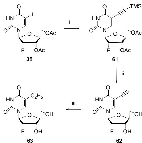
Scheme 6. Reagents and conditions: (i) Et 3 N, CuI, (Ph 3 P) 2 PdCl 2 , TMSCH, 50–60 °C, 7 h; (ii) NaOMe, MeOH, rt, 15 h; (iii) EtOH, 10% Pd-C, H 2 , 1 atm, 1 h.
