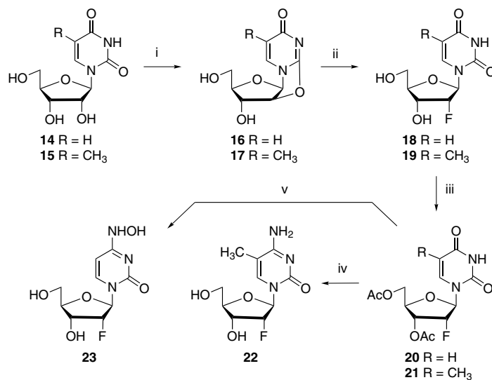
Scheme 3. Reagents and conditions: (i) HMPA, Ph 2 CO, NaHCO 3 , 150 °C, 30 min; (ii) HF–pyridine, dioxane, 120–125 °C, 18 h; (iii) Ac 2 O, pyridine; (iv) (a) CH 3 CN, Et 3 N, TIPCl, DMAP, rt, 1 d; (b) NH 4 OH, rt, 1 d; (v) (a) CH 3 CN, Et 3 N, TIPCl, DMAP, rt, 1 d; (b) NH 2 OH·HCl, rt, 1 d; (c) NH 3 /MeOH, rt, 14 h.
